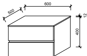
2DR600
