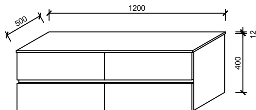
2x2DR600
