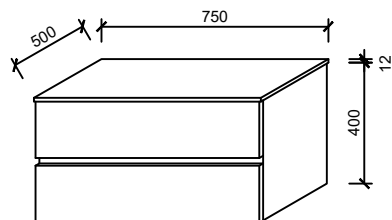
2DR750
