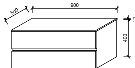
2DR900
