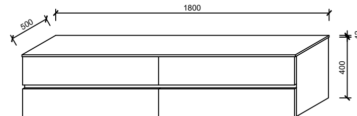
2x2DR900
